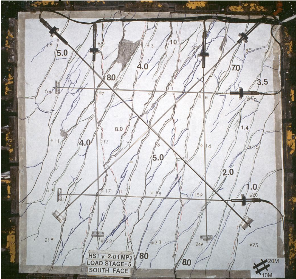
HS1: Load Stage 5 and final state: South Face
